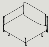
HA1-R/L-LOFT* W 910 D 910 H 750 S 410 W 35.8" D 35.8" H 29.5" S 16.2"
