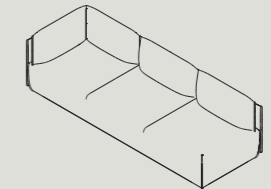
HCA3-R/L* W 2570 D 910 H 750 S 410 W 101.2" D 35.8" H 29.5" S 16.2"
