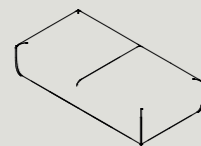
HO2 W 1660 D 830 H 410 W 65.4" D 32.7" H 16.2"
