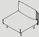
HB1-LOFT W 830 D 910 H 750 S 410 W 32.7" D 35.8" H 29.5" S 16.2"
