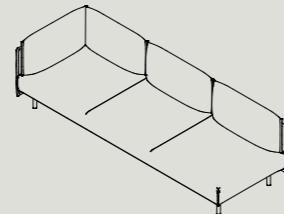
HCA3-R/L-LOFT* W 2570 D 910 H 750 S 410 W 101.2" D 35.8" H 29.5" S 16.2"
