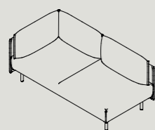
HCA2-R/L-LOFT* W 1740 D 910 H 750 S 410 W 68.5" D 35.8" H 29.5" S 16.2"
