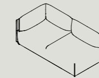
HCA2-R/L* W 1740 D 910 H 750 S 410 W 68.5" D 35.8" H 29.5" S 16.2"
