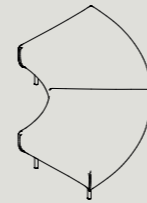
HO45D-LOFT W 1685 D 1685 H 410 IN Ø1700 / OUT Ø3340 W 66.3" D 66.3" H 16.2" IN Ø67" / OUT Ø131.5"
