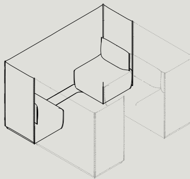
PHB-HUB-SC-2340 W 730 D 2340 H 1350 S 440 W 28.7" D 92.1" H 53.1" S 17.3"
