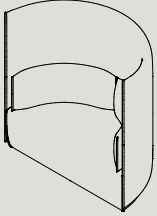
PHL2-ARC W 1460 D 730 H 1350 S 440 OUT Ø1460 W 57.5" D 28.7" H 53.1" S 17.3" OUT Ø57.5"
