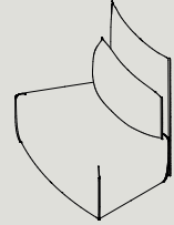
PMB30-R W 1090 D 920 H 1025 S 440 IN Ø2920 / OUT Ø4380 W 42.9" D 36.2" H 40.4" S 17.3" IN Ø115.0" / OUT Ø172.4"
