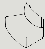
PB30-R W 1090 D 920 H 760 S 440 IN Ø2920 / OUT Ø4380 W 42.9" D 36.2" H 30.0" S 17.3" IN Ø115.0" / OUT Ø172.4"
