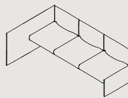
DEA3-IND-S/W-R/L* W 2110 D 1115/1190 H 740 S 440
