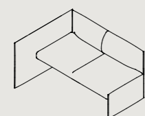
DEA2-S/W-R/L* W 1450 D 1115/1190 H 740 S 440
