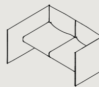
DEL2-S/W-IND-R/L* W 1450 D 1115/1190 H 740 S 440
