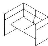
DMEL2-S/W-R/L* W 1450 D 1115 / 1190 H 1020 S 440
