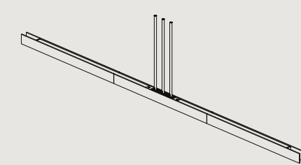
LP.2510.TD L2510 W48 H64 / L98.8" W1.9" H2.5" MIN DROP HEIGHT - H300 / 11.8"
