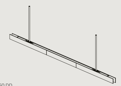
LP.1950.DD L1950 W48 H64 / L76.8" W1.9" H2.5" MIN DROP HEIGHT - H300 / 11.8" CEILING CANOPY SPACING - 1260MM / 49.61"
