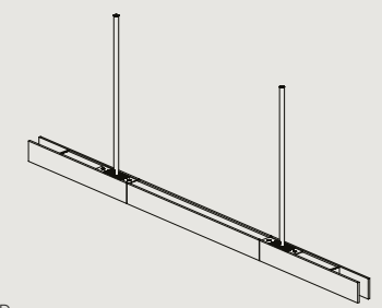
LP.1390.DD L1390 W48 H64 / L54.7" W1.9" H2.5" MIN DROP HEIGHT - H300 / 11.8" CEILING CANOPY SPACING - 700MM / 27.56"
