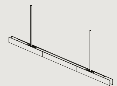
LP.1670.DD L1670 W48 H64 / L65.7" W1.9" H2.5" MIN DROP HEIGHT - H300 / 11.8" CEILING CANOPY SPACING - 980MM / 38.58"
