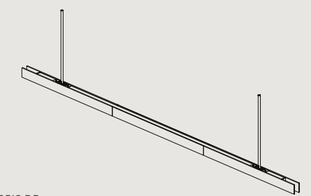
LP.2510.DD L2510 W48 H64 / L98.8" W1.9" H2.5" MIN DROP HEIGHT - H300 / 11.8" CEILING CANOPY SPACING - 1820MM / 71.65"
