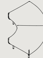
HO45D-LOFT W 1685 D 1685 H 410 IN Ø1700 / OUT Ø3340
