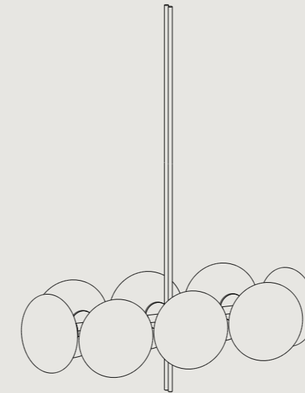
AE108 L 980 W 460 H 350 L 38.6" W 18.1" H 13.8" MIN DROP HEIGHT - H 600 / 23.6"
