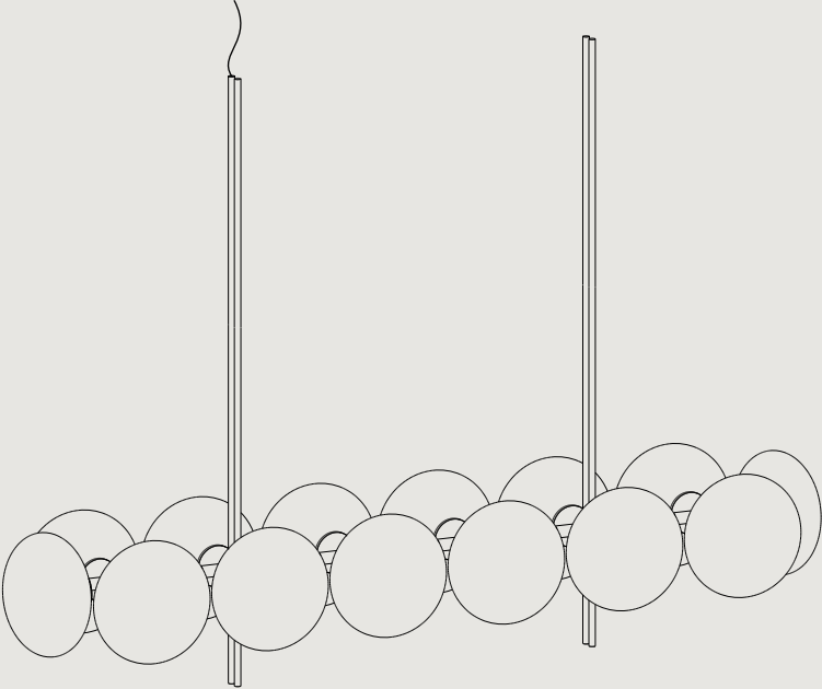
AE214 L 1760 W 460 H 350 L 69.3" W 18.1" H 13.8" MIN DROP HEIGHT - H 600 / 23.6" CEILING CANOPY SPACING L780MM / 30.7"
