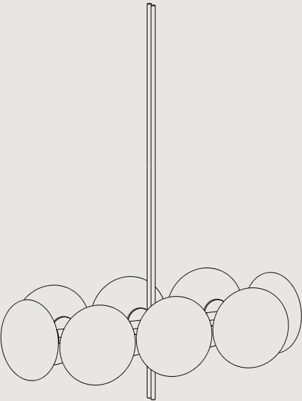
AE108 L 980 W 460 H 350 L 38.6" W 18.1" H 13.8" MIN DROP HEIGHT - H 600 / 23.6"
