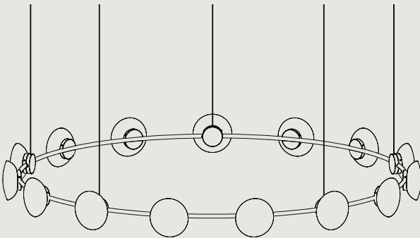
CC2015 - INDIVIDUAL CANOPY Ø 2175 H 200 RING Ø 2000 Ø 7'2" H 7.9" RING Ø 6' 7" MIN DROP HEIGHT - H 600 / 2'
