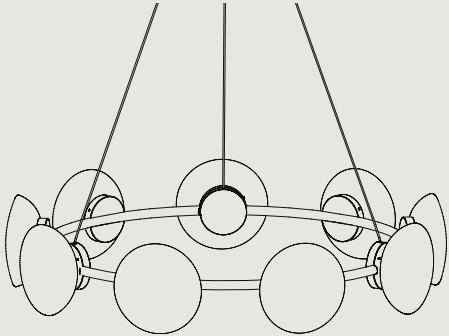
CC809 - CENTRAL CANOPY Ø 980 H 200 RING Ø 800 Ø 3'3" H 7.9" RING Ø 2'75" MIN DROP HEIGHT - H 600 / 2'
