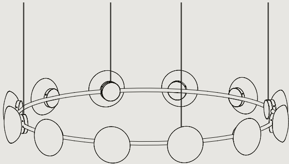
CC1412 - INDIVIDUAL CANOPY Ø 1675 H 200 RING Ø 1400 Ø 5'2" H 7.9" RING Ø 4' 7" MIN DROP HEIGHT - H 900 / 2'
