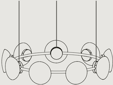
CC809 - INDIVIDUAL CANOPY Ø 980 H 200 RING Ø 800 Ø 3'3" H 7.9" RING Ø 2'75" MIN DROP HEIGHT - H 600 / 2'
