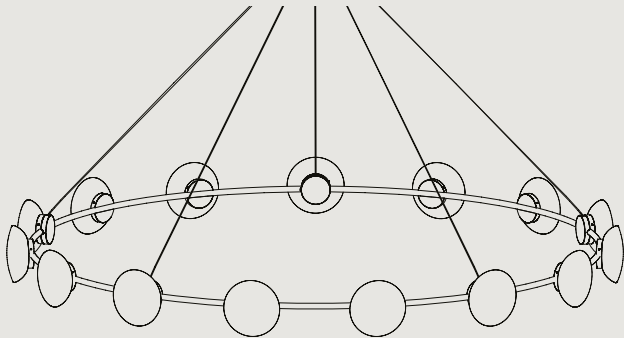
CC2015 - CENTRAL CANOPY Ø 2175 H 200 RING Ø 2000 Ø 7'2" H 7.9" RING Ø 6' 7" MIN DROP HEIGHT - H 1200 / 3'11"
