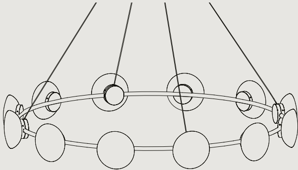
CC1412 - CENTRAL CANOPY Ø 1675 H 200 RING Ø 1400 Ø 5'2" H 7.9" RING Ø 4' 7" MIN DROP HEIGHT - H 900 / 2'11"
