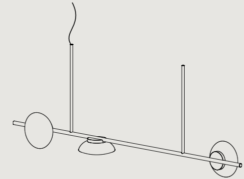
CH23L* L 1706 W 200 H 200^ L 67.2" W 7.9" H 7.9"^^ CEILING CANOPY SPACING L 840MM / 17.32"
