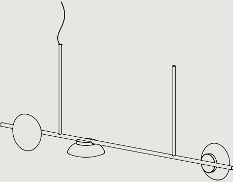
CH23L* L 1706 W 200 H 200^ L 67.2" W 7.9" H 7.9"^ CEILING CANOPY SPACING L 840MM / 17.32"
