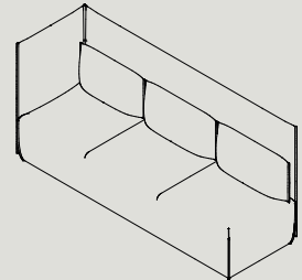
PMA3-R/L* W 2190 D 730 H 1025 S 440 W 86.2" D 28.7" H 40.4" S 17.3"
