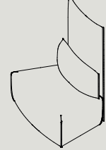
PHB30-R W 1090 D 920 H 1350 S 440 IN Ø2920 / OUT Ø4380 W 42.9" D 36.2" H 53.1" S 17.3" IN Ø115.0" / OUT Ø172.4"
