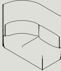
PHL2-ARC-HLF-L/R* W 1460 D 730 H 1350 S 440 W 57.5" D 28.7" H 53.1" S 17.3"
