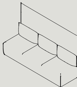
PHB3 W 2190 D 730 H 1350 S 440 W 86.2" D 28.7" H 53.1" S 17.3"
