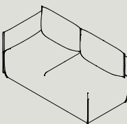
PA2-R/L* W 1460 D 730 H 760 S 440 W 57.5" D 28.7" H 30.0" S 17.3"
