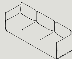
PL3 W 2190 D 730 H 760 S 440 W 86.2" D 28.7" H 30.0" S 17.3"
