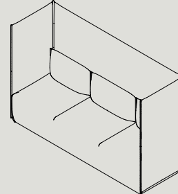
PHL3 W 2190 D 730 H 1350 S 440 W 86.2" D 28.7" H 53.1" S 17.3"
