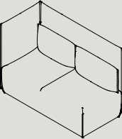
PMA2-R/L* W 1460 D 730 H 1025 S 440
