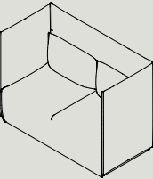
PML2 W 1460 D 730 H 1025 S 440
